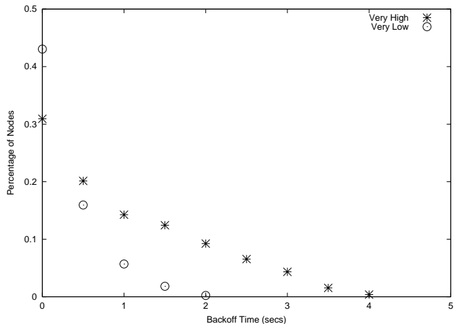
Figure 10: Distribution of backoff delay before successful transmission at two transmission power settings.
