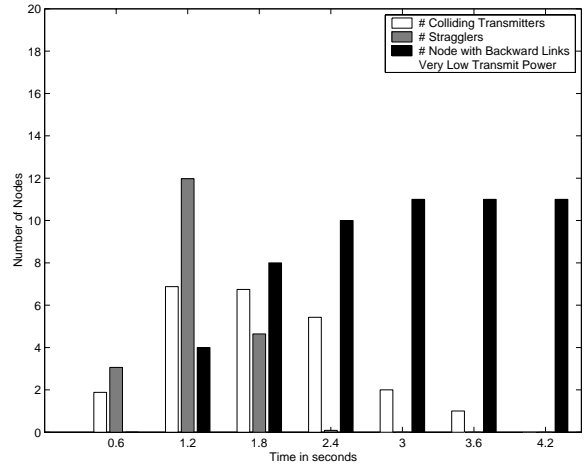
(b) Very Low transmit power setting.
