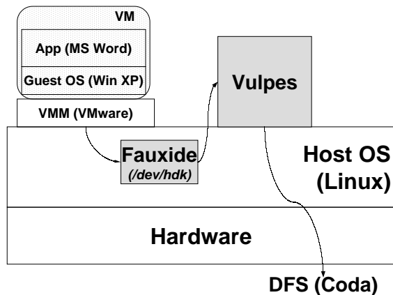
Figure 1. ISR Host Architecture
